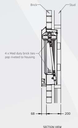
SECTION VIEW
